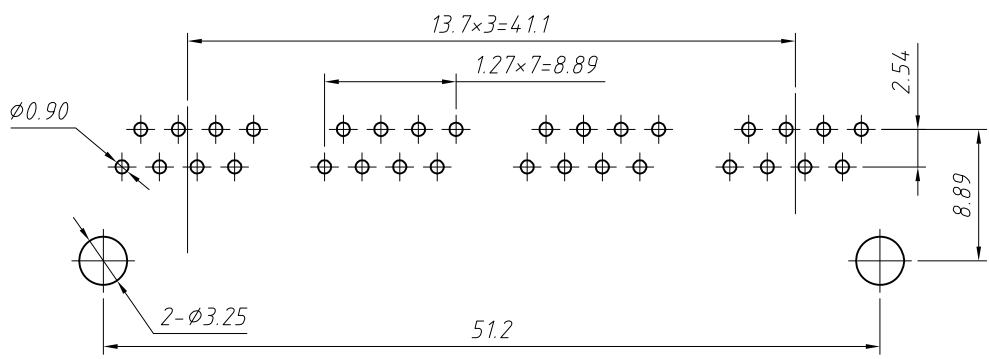
PCB Layout
